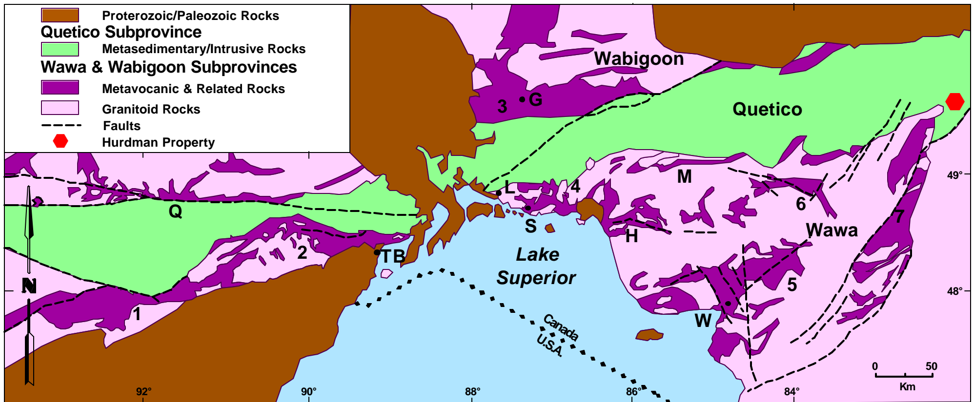
Figure 1. Tectonic map showing the Wawa, Quetico, and southern Wabigoon subprovinces of the south-central Superior Province.
